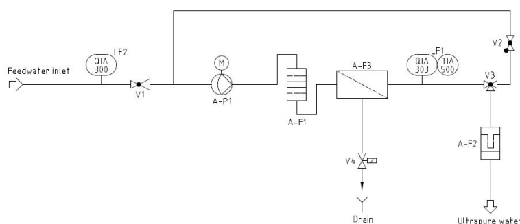
Flow chart for MicroPure UF
